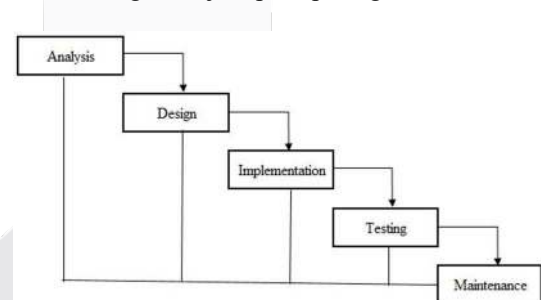
GAMBAR 1 Model Waterfall
