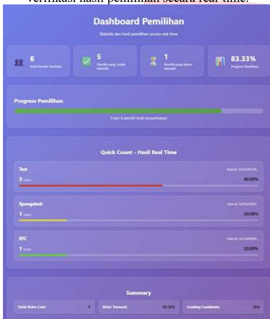
GAMBAR 17 Dashboard Admin
