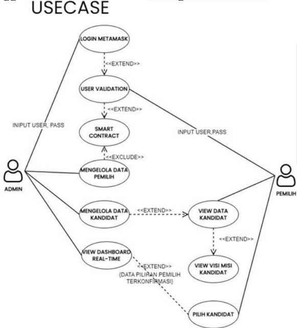
GAMBAR 2 Use Case E-Voting
