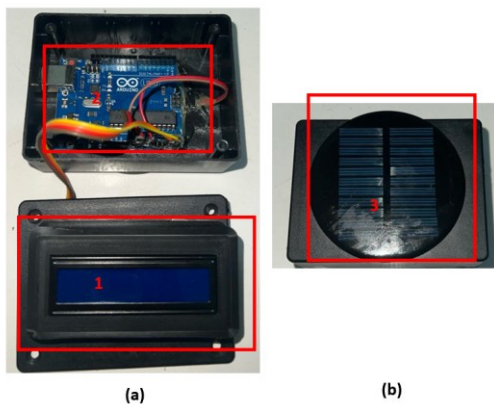
GAMBAR 7 HASIL PERANCANGAN RECEIVER LI-FI
