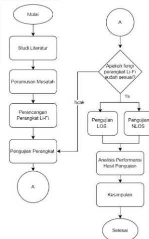
GAMBAR 3 ALUR PENELITIAN
