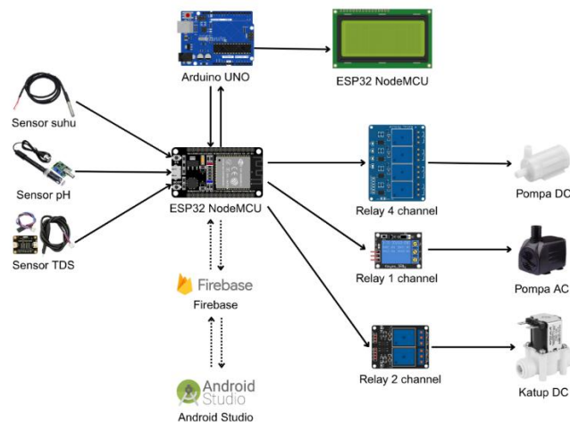
Gambar 1. Desain Sistem IoT Smart Farming
