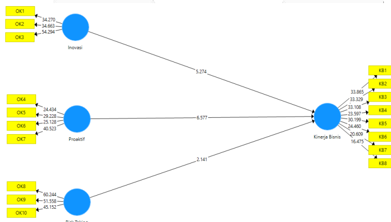
Gambar 4.4 Path Diagram Inner Model
