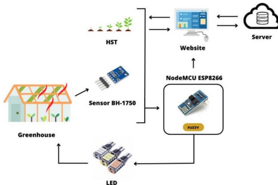
Gambar 1.4 Alur Diagram Sistem
