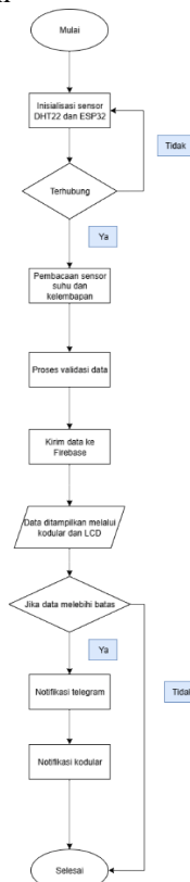
GAMBAR 3 Flowchart Diagram
