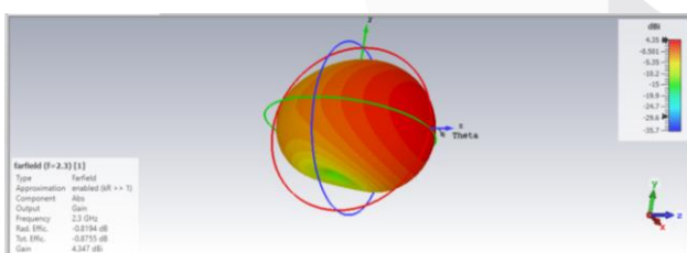
Gambar 10 (Hasil gain rancangan antenna)
