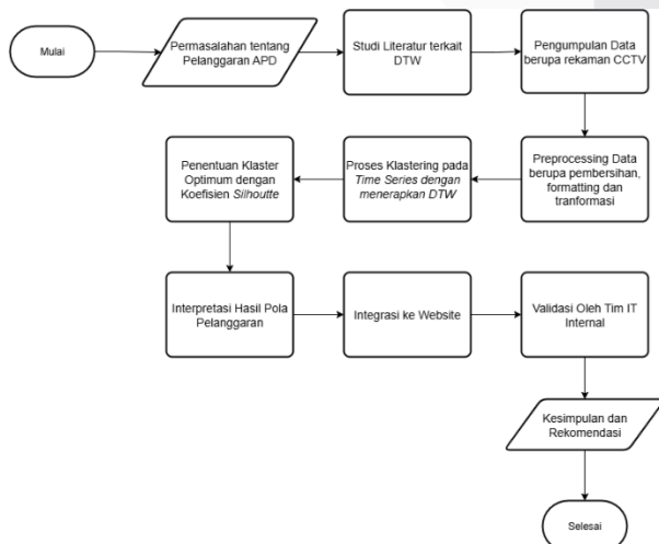
Gambar 1 Flowchart Penelitian
