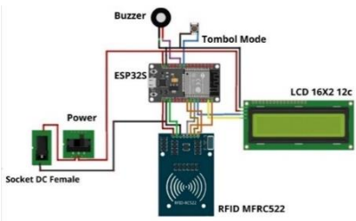
Gambar 6 Blok diagram
