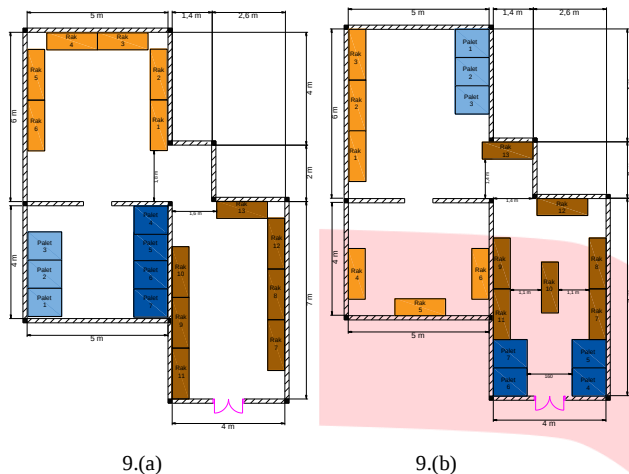
9.(a) 9.(b) GAMBAR 9 Layout Eksisting, Layout Usulan I, dan Layout Usulan II
