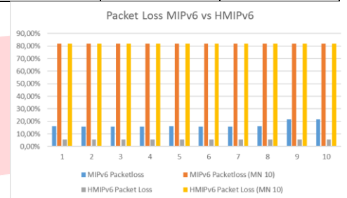
Gambar 2 Grafik Packet Loss
