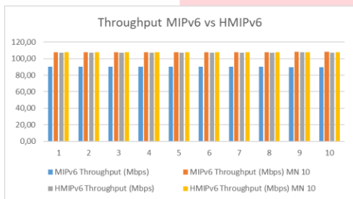
Gambar 3 Grafik Throughput
