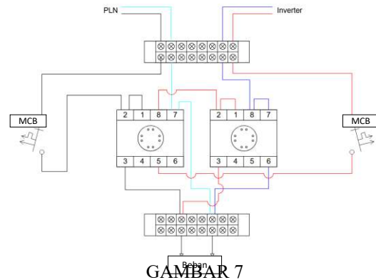
GAMBAR 7 Sistem Automatic Transfer Switch (ATS)
