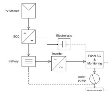
GAMBAR 8 Wiring diagram
