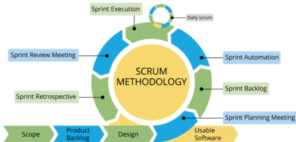
Gambar 1. 1 Scrum Methodology
