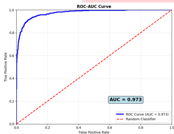
Gambar 4 ROC-AUC Curve BiLSTM
