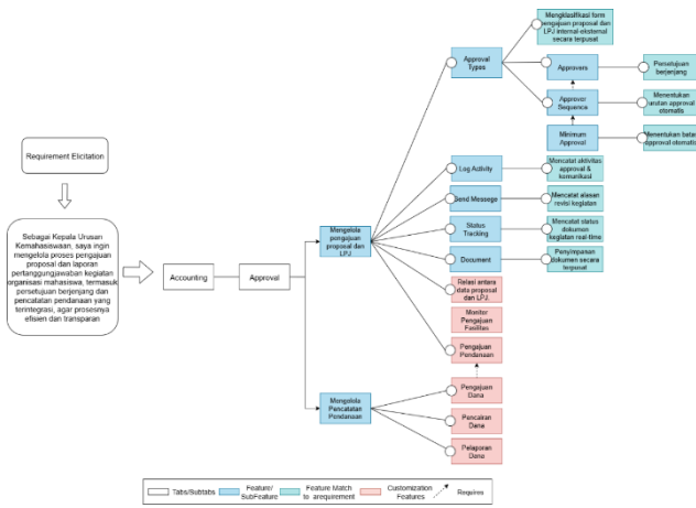
GAMBAR 6 (Feature Model)
