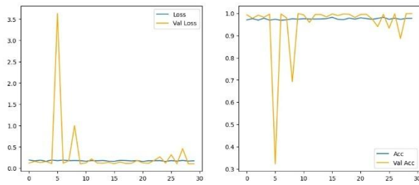
GAMBAR 2 (Grafik Hasil Training Loss dan Accuracy )
