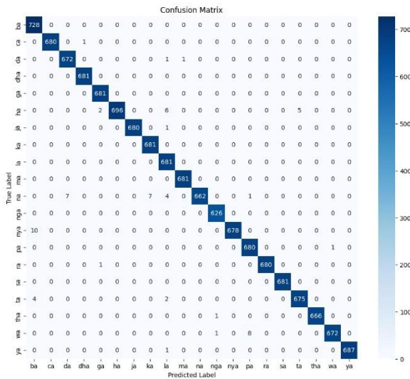
GAMBAR 3 ( Confusion Matrix )
