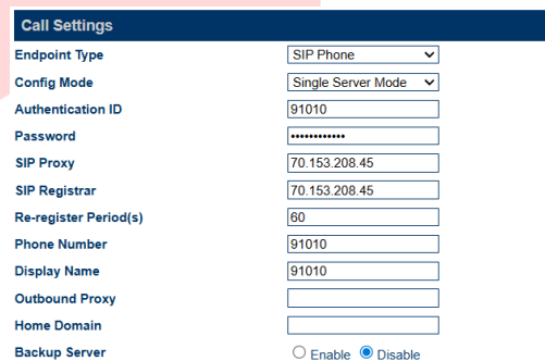
Gambar 5 Integrasi GSM Gateway
