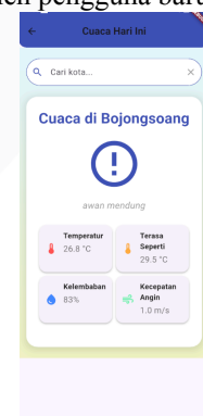
GAMBAR 7 (halaman OpenWeather)
