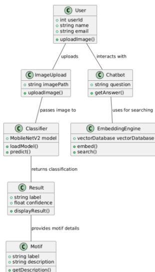
GAMBAR 9 (Class Diagram)
