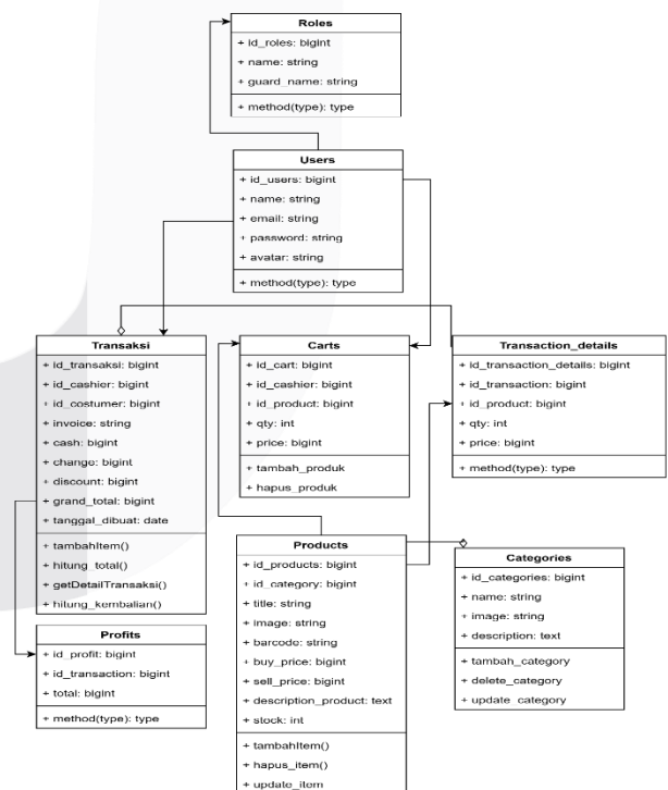
GAMBAR 4 (Class Diagram)
