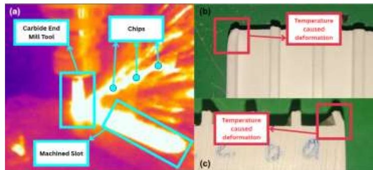
Figure I-1 Thermal and physical signs of overheating during machining.
