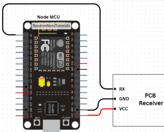
GAMBAR 9 Skematik Receiver
