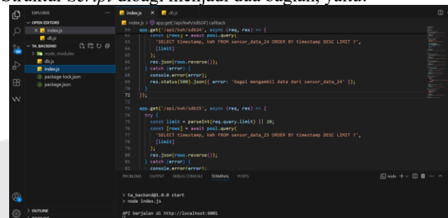
Gambar 4. 1 Script Backend
