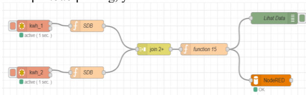
Gambar 4. 3 Flow SDB 1
