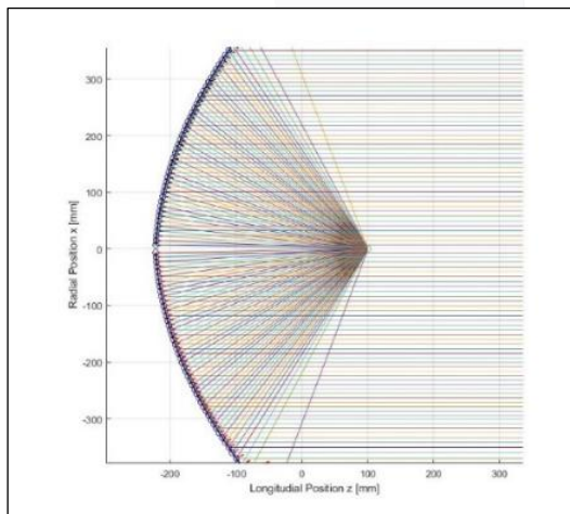
Gambar 5 Ray Tracing
