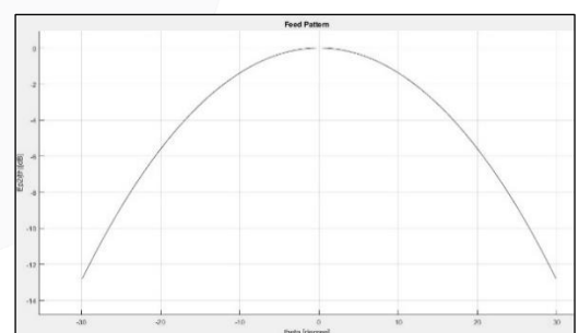
Gambar 8 Polaradiasi Feed
