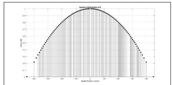
Gambar 6 Distribusi Aperture
