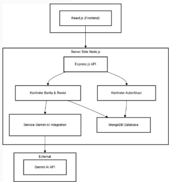
Gambar 7 Component Diagram
