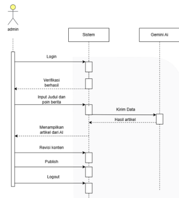
Gambar 5 Sequence Diagram
