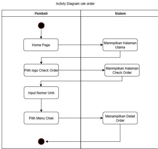
Gambar 3. 4 Activity diagram cek order
