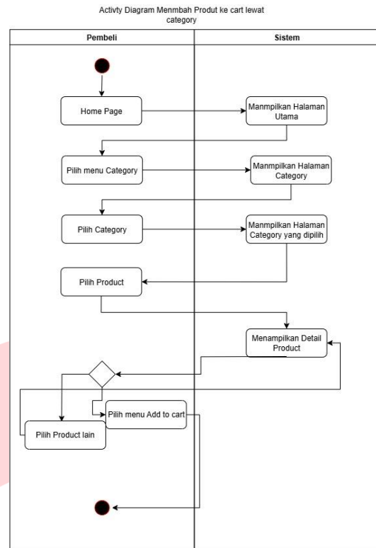
Gambar 3. 2 Activity diagram menambah product ke cart lewat category
