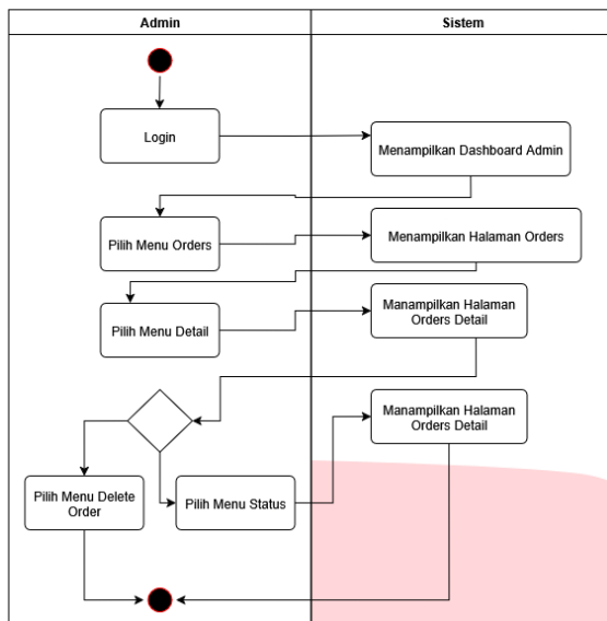
Gambar 3. 8 Activity diagram admin mengubah status order
