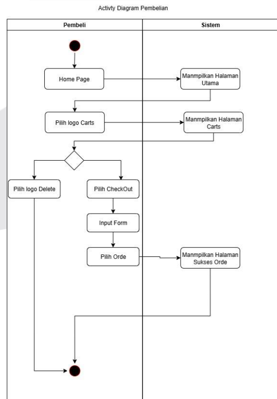
Gambar 3. 3 Activity diagram pembelian
