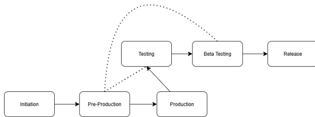
Gambar 1 Diagram GDLC
