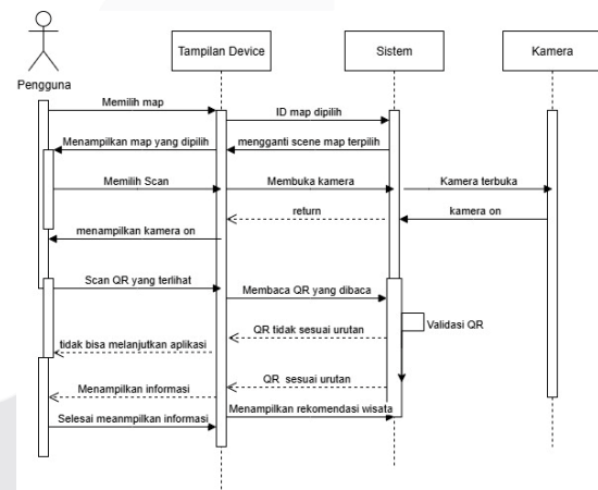
Gambar 4 Sequence Diagram
