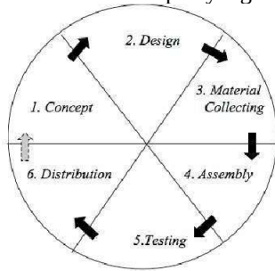
GAMBAR 1 Metode MDLC
