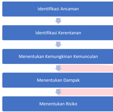
Gambar 1. Tahapan NIST SP 800-30 Rev 1 [8]
